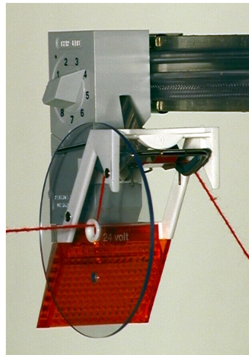
330.000.015.01 top detector FW, 12V, 1,2kOhm for installation to the tube duct at the tube input
