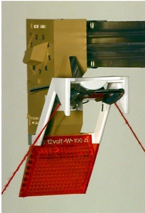
330.000.002 top detector OFW, 12V, 100 Ohm
